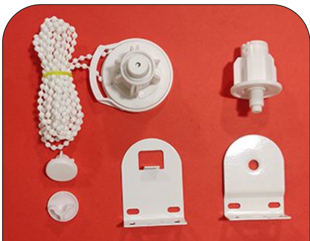
HT-38C003 UNIVARSAL CONTROL UNIT
